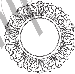
RMF 7039 RING 12-3/16" O. DIA. x 5/8"D 6-7/16" I. DIA.
